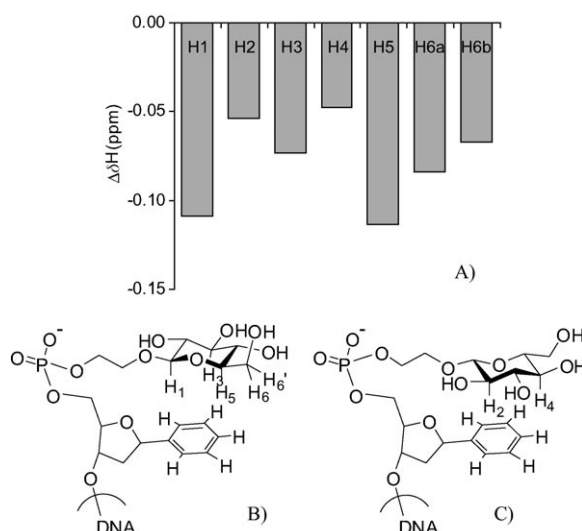
Figure 3. A) Upfield shifting of carbohydrate protons due to the proximity to the face of the aromatic ring. Differences are calculated between the conjugate containing \beta -D-glucose on the sequence BCGCGCG, 3 , and 2-hydroxyethyl- \beta -D-glucopyranoside ( 8 ). B) Model of possible stacking geometry of \beta -glucose on top of the benzene ring through the \alpha face of the sugar. C) Model of possible stacking geometry of \beta -glucose on top of the benzene ring through the \beta face of the sugar.
