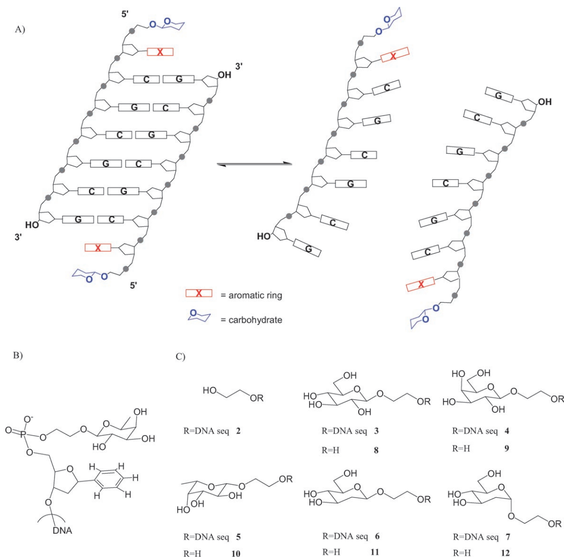
Scheme 1. A) Dangling-ended DNA model system designed to measure carbohydrate–aromatic interactions. B) Enlarged view of the structure of the dangling-end area of the carbohydrate–oligonucleotide conjugate. C) Carbohydrate–oligonucleotide conjugates included in the study. Oligonucleotide conjugate 1 is BCGCGCG, in which B is the benzene nucleoside. In conjugates 2–7 , DNA seq represents OPO _2 –BCGCGCG.
