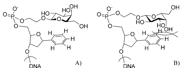
Figure 1. Model of the dangling-end area of carbohydrate–DNA conjugate 4 , which contains a \beta -galactose unit. A) Possible stacking geometry of \beta -galactose on top of the benzene ring through the \alpha face of the sugar. B) Possible stacking geometry of \beta -galactose on top of the benzene ring through the \beta face of the sugar, with the steric clash between the 4-OH group and the arene shown.
