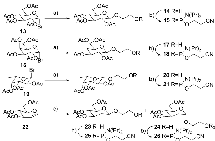
Scheme 2. Synthetic routes used to prepare the carbohydrate phosphoramidite derivatives. a) Ethylene glycol, \text{Ag}_2\text{CO}_3 , \text{CH}_2\text{Cl}_2 , RT, 18 h, 28–62%; b) 2-cyanoethyl- N,N' -diisopropylamino-chlorophosphoramidite, N,N' -diisopropylethylamine (DIEA), \text{CH}_2\text{Cl}_2 , RT, 1.5 h, 74–92%; c) ethylene glycol, \text{PPh}_3\text{HBr} , \text{CH}_2\text{Cl}_2 , RT, 7 h, 5% of 23 and 20% of 24 .
